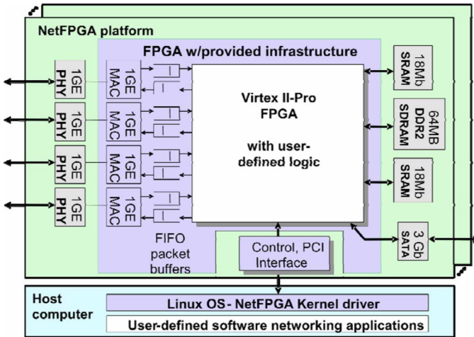
Fig. 3. Block diagram of the NetFPGA.
