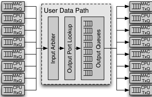
Fig. 5. NetFPGA's router data path.
