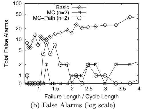
Figure 8: Effect of aggregation strategies on tomography, 0.6% of detection errors.
